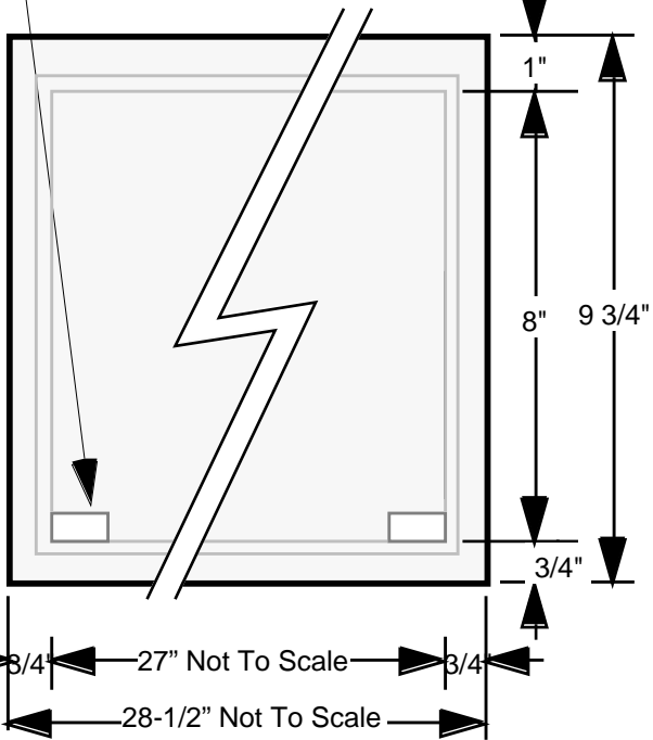
ROOF—LOOKING DOWN AT TOP
