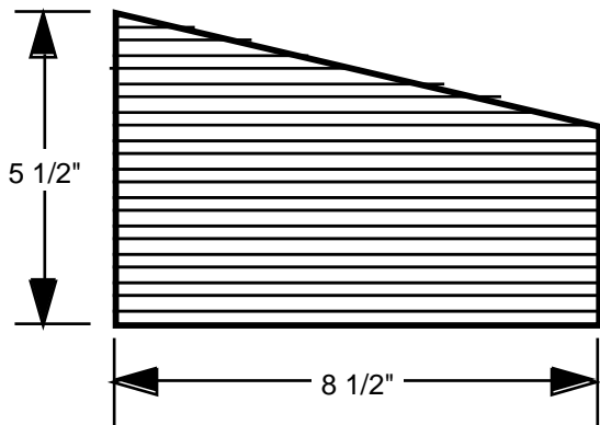
REAR END PIECE
