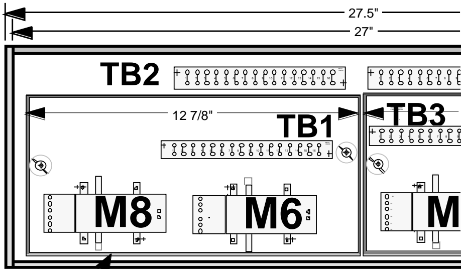
TOP VIEW —ROOF REMOVED
